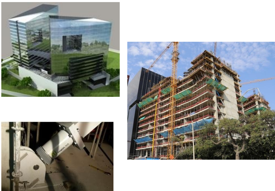
Fig. 9 “Panorama business center” tower buildings in Lima, Peru
