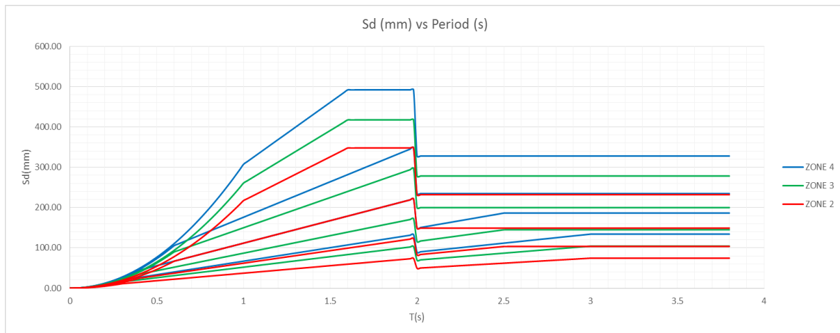
Fig. 6 Displacement spectra according to the Peruvian seismic code (2016)
